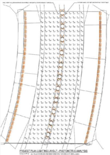
Column Photometrics
